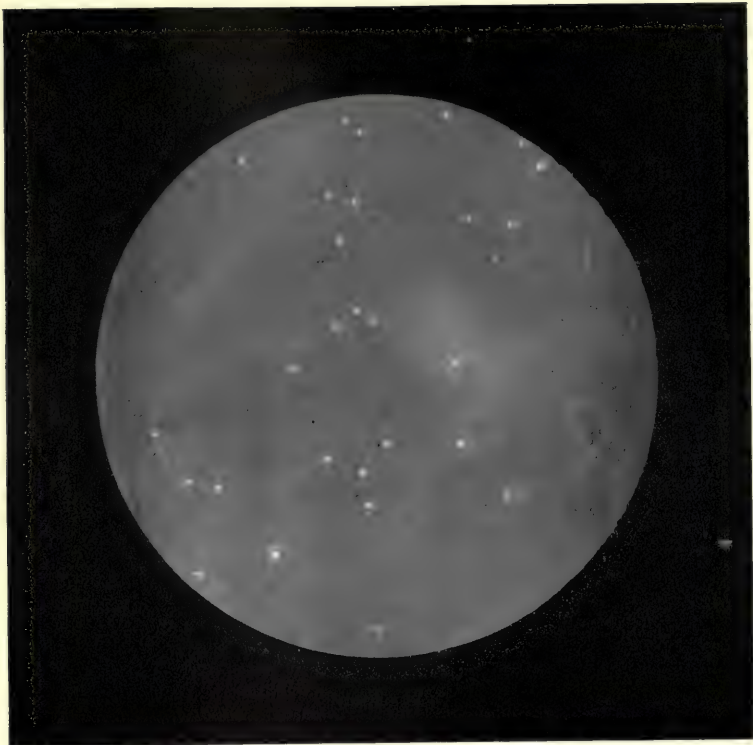
ENCKE'S COMET.
